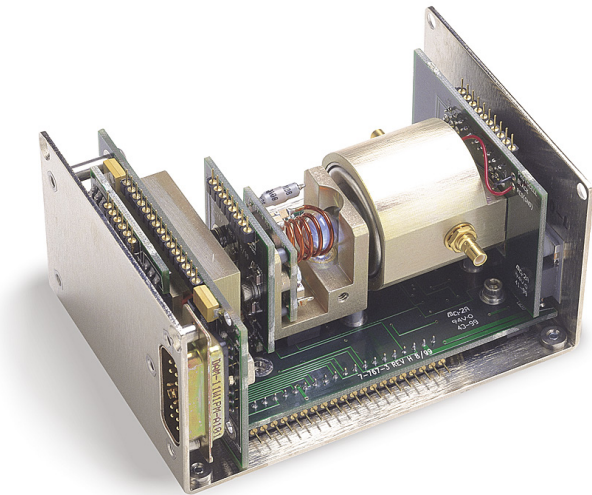
PRS10 physics package and lamp assembly
