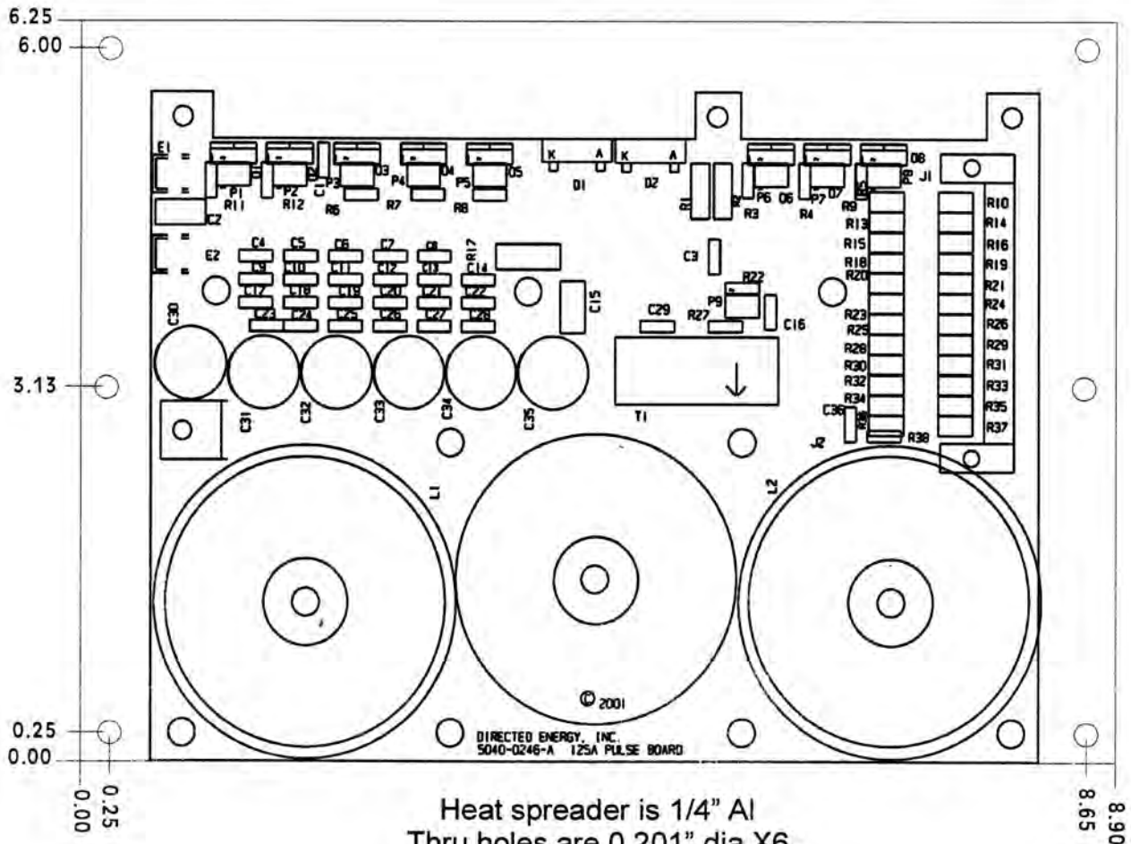
PCO-6141 Dimensional Drawing
