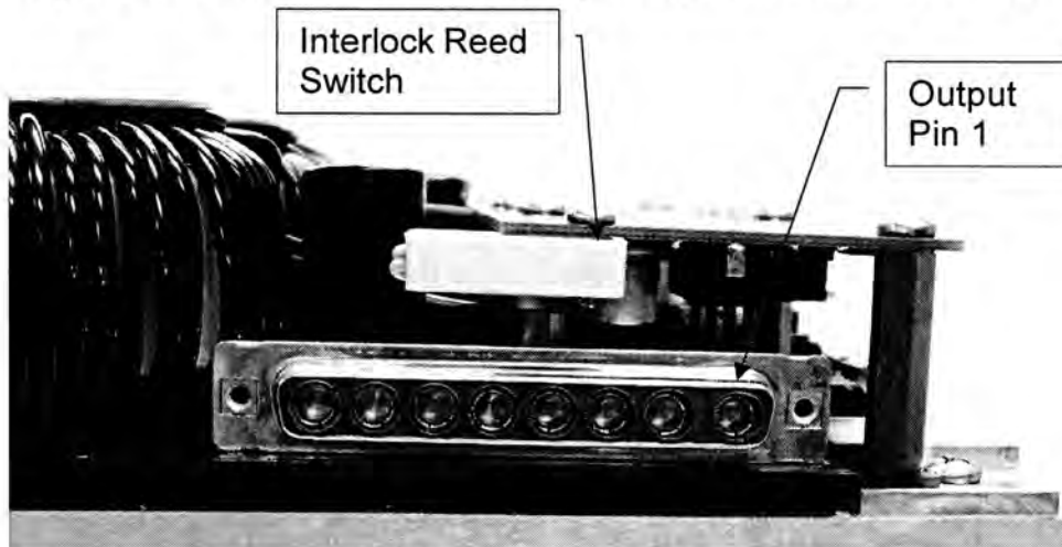
Figure 2A: Magnetic Interlock, Output Connector Pin 1
