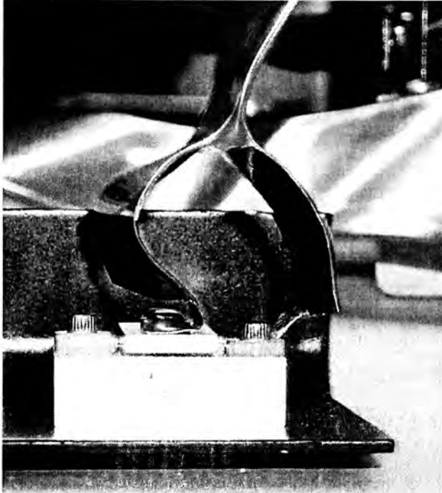
Figure 4 - Stripline Connection To Laser Diode
