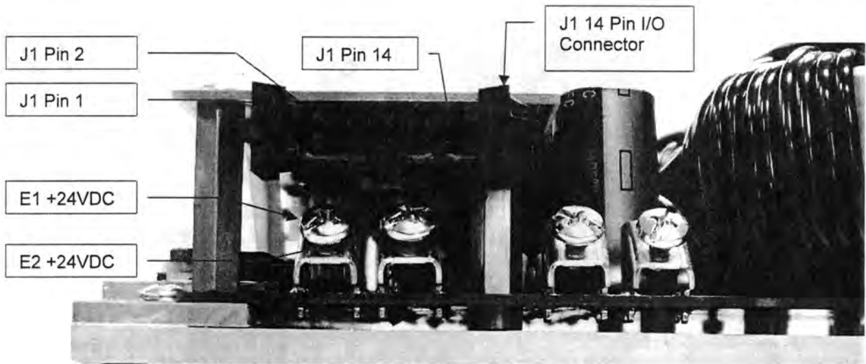
Figure 1: Connectors J1, E and E2 Locations
